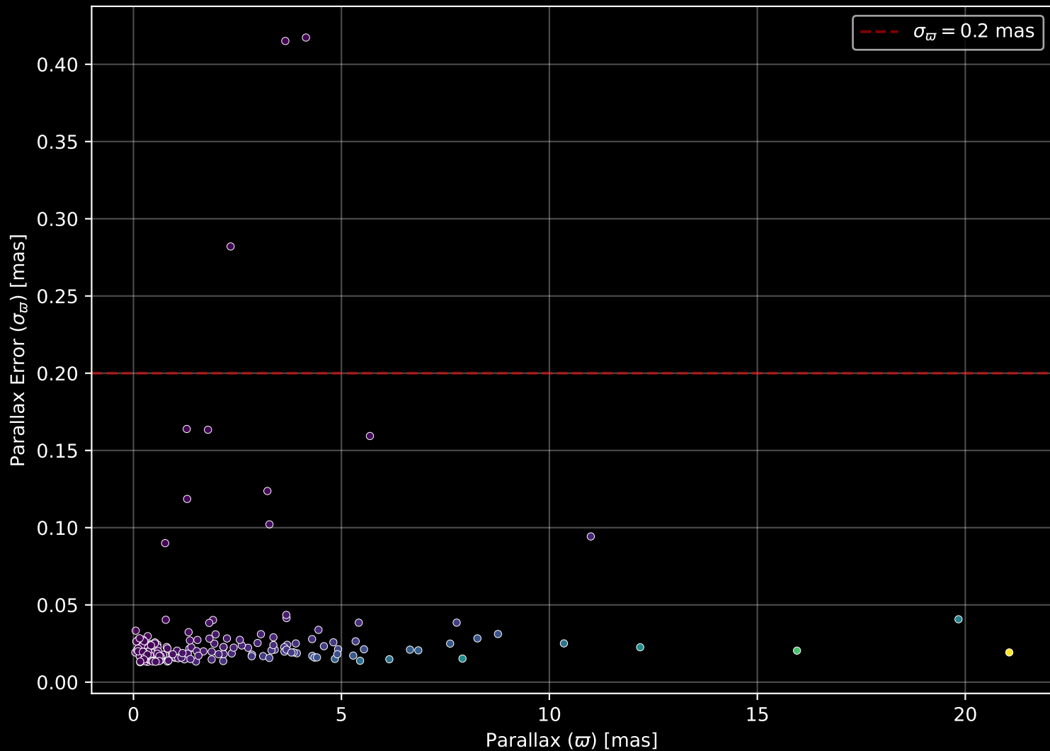
APOGEE DR17 Field: [010+60] Parallax Quality (n= 190)
