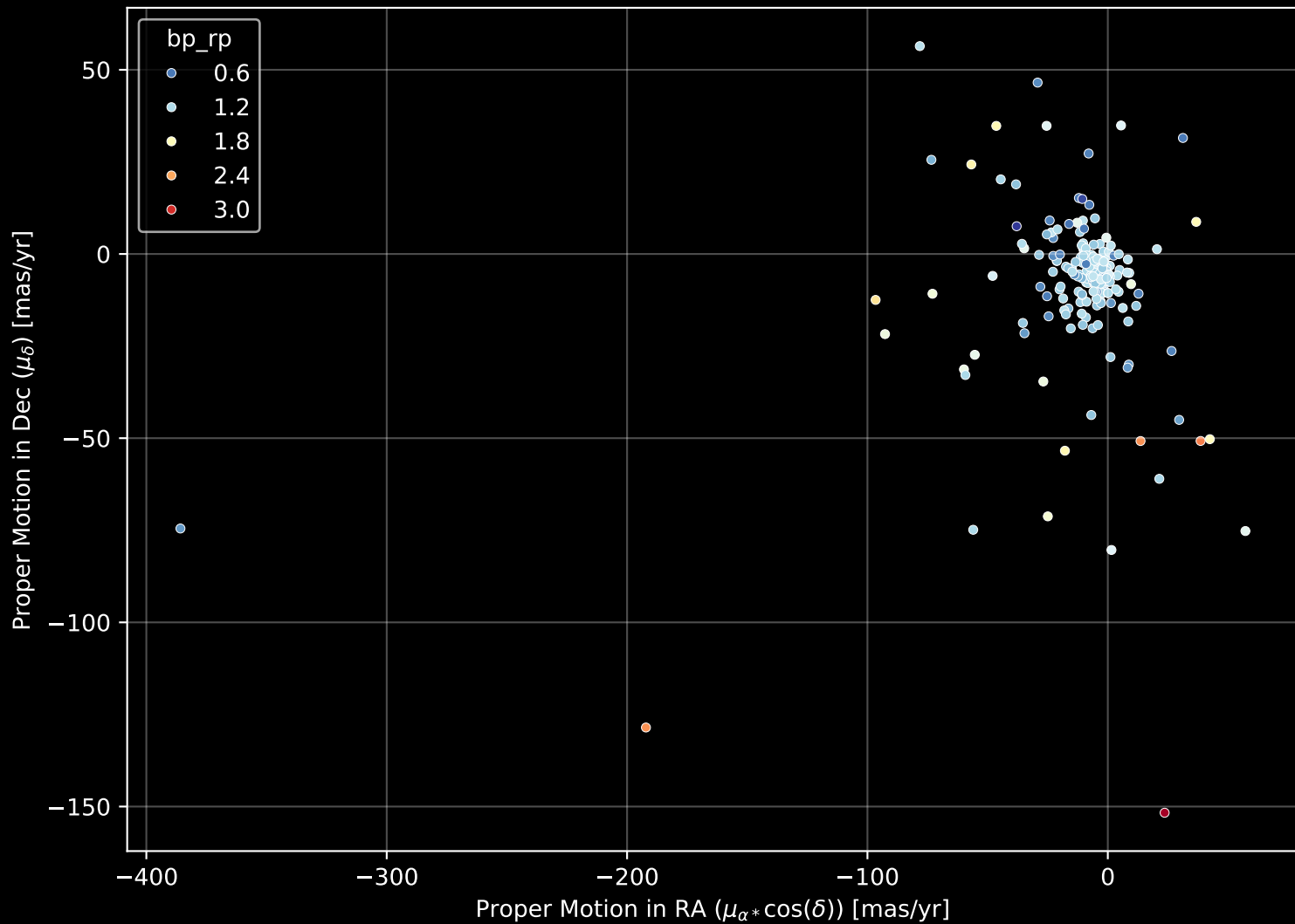
APOGEE DR17 Field: [010+60] Proper Motion Diagram (n= 190)
