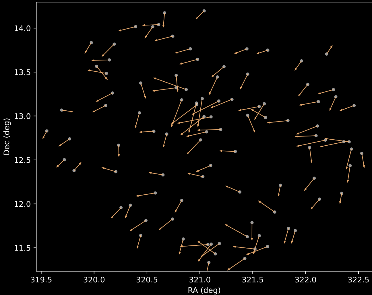
APOGEE DR17 Cluster 3 Proper Motion Vectors (n=97)
