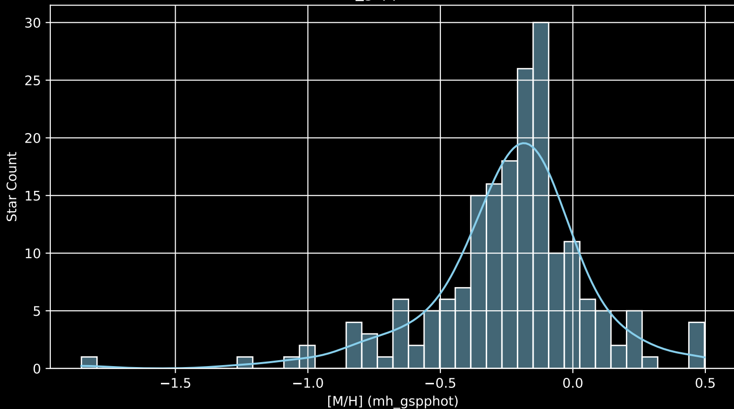
APOGEE DR17 Field: [010+60 [M/H] (mh_gspphot) (n= 188)
