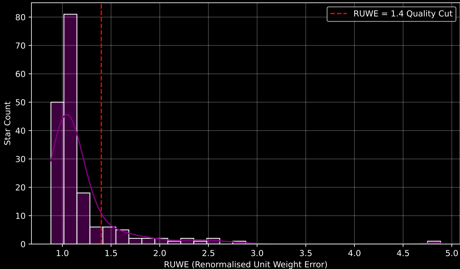
GAPOGEE DR17 Field [010+60] RUWE Distribution (n= 180)
