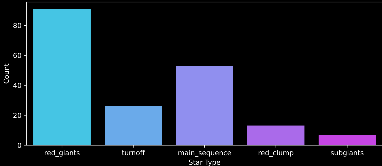
APOGEE DR17 Field: [010+60] Count plot of Star Type
